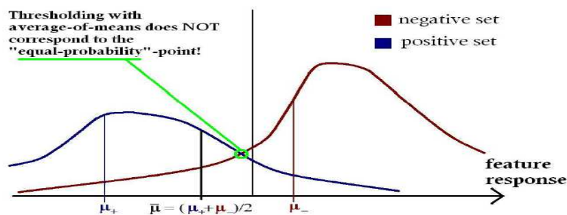
Figure 2.6: An example of how the distribution of feature values for a specific feature may look like over the set of all training samples.
