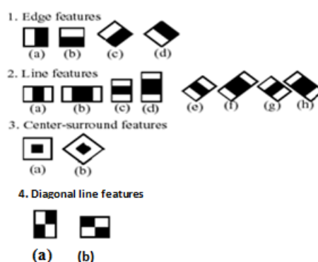
Figure 2.2: A set of extended Haar-like features.
