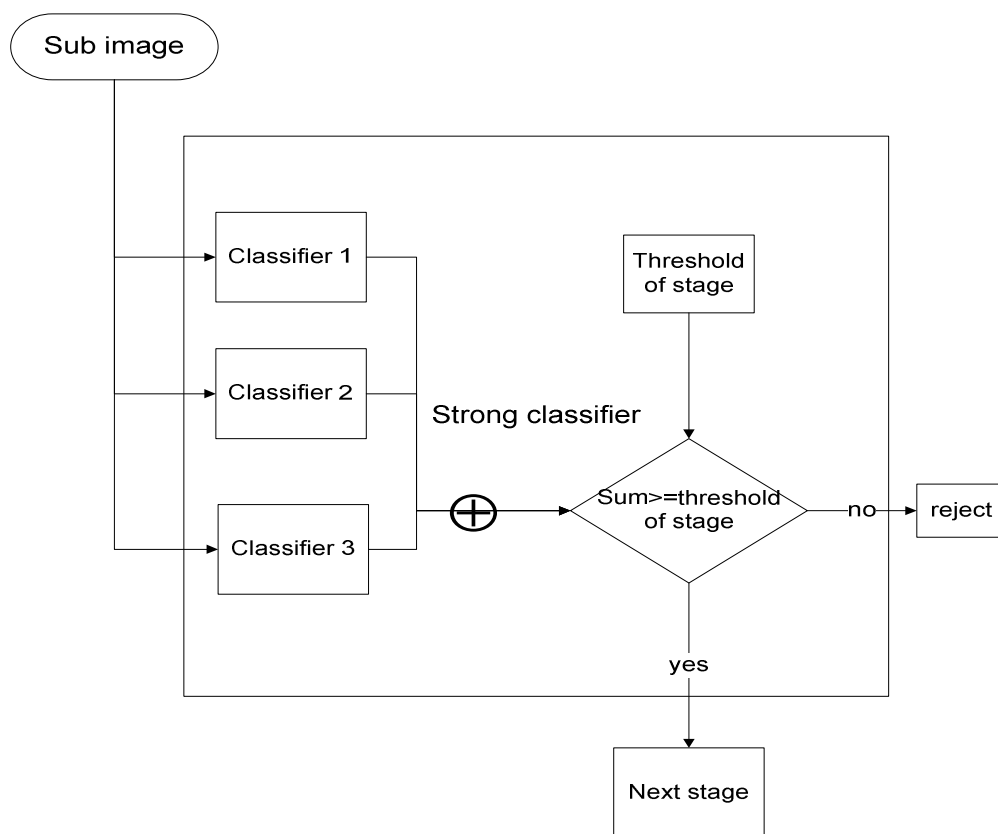
Figure 3.9: The detection procedure.
