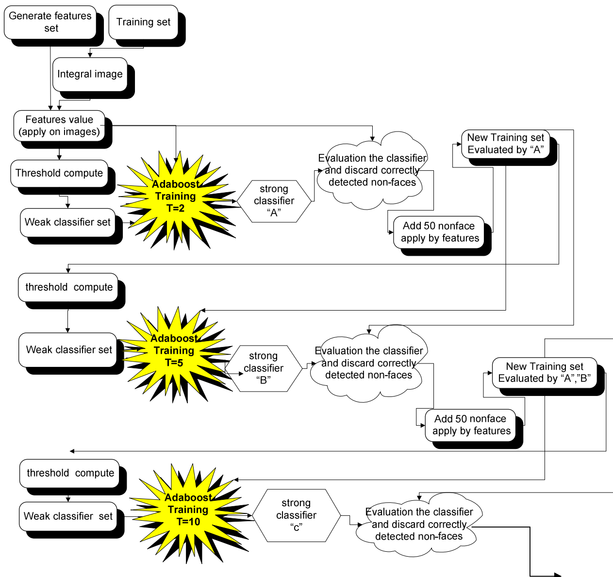
Figure 3.1: The Cascade Training Process for three stages.
