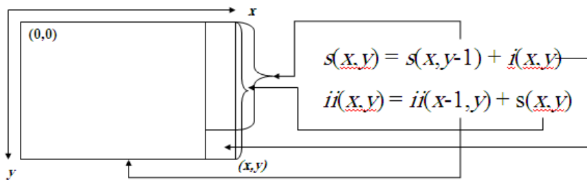
Figure 2.4: The Integral Image Calculation Process
