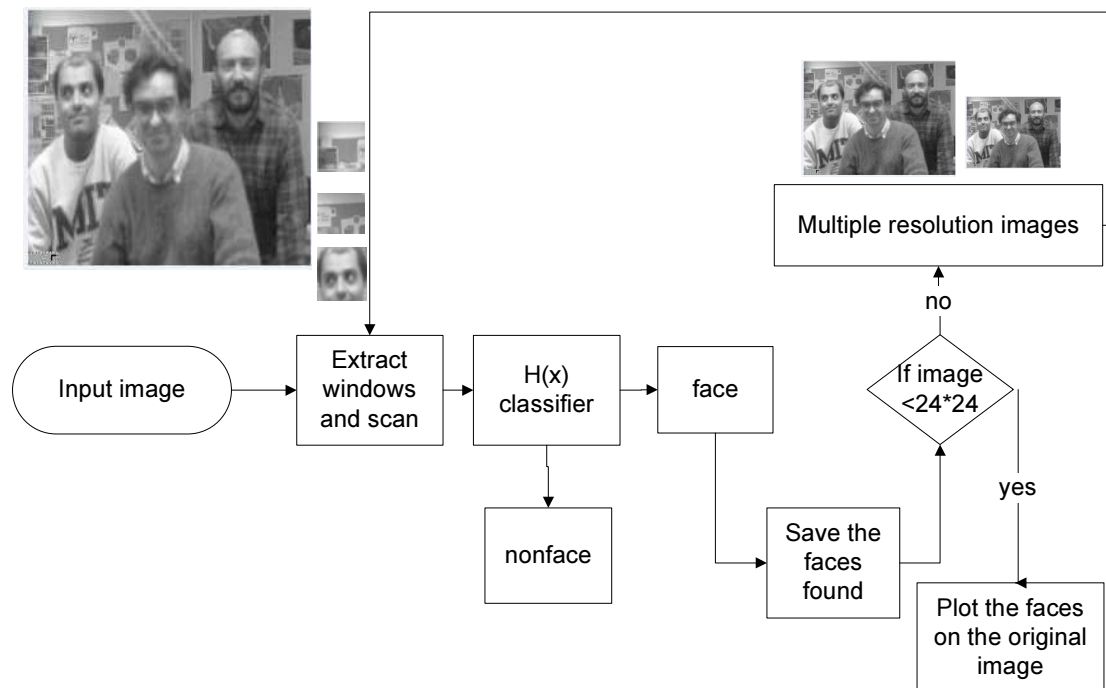
Figure 3.10: The block diagram of the face detector used in the system.
