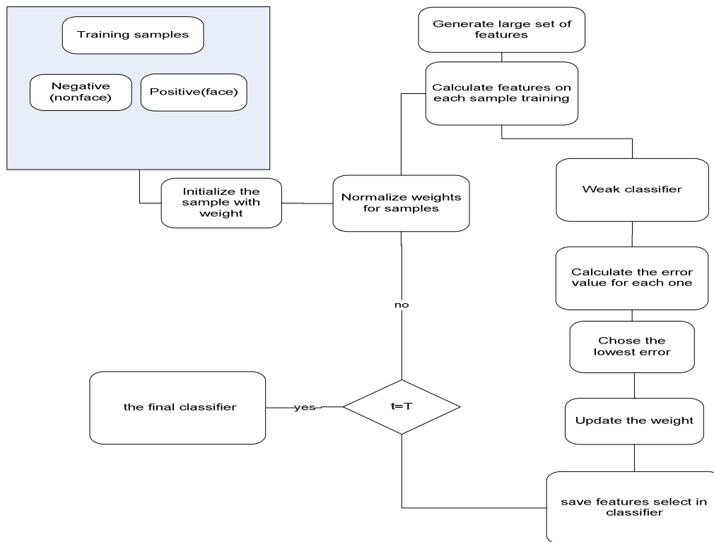
Figure 3.7: the Adaboost training diagram explains how the Adaboost algorithm works.
