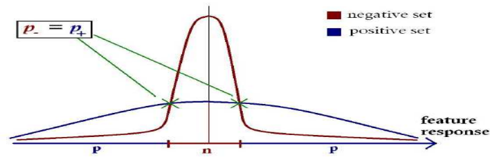
Figure 2.9: By parameterizing the two distributions with a Gaussian model, one can find the two intersection points that will represent the two thresholds. The parameterized approach is less sensitive to noise than statistics/numerical ways to find the two intersecting points of the histogram plots
