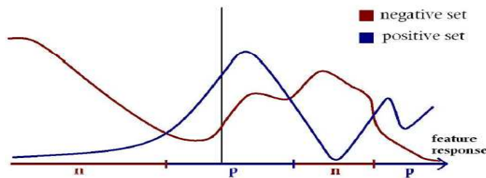
Figure 2.10: This figure illustrates the case of multimodal PDFs (given by feature f_i ) for the positive and negative training set. By following the largest probability while classifying, one can adapt the multi-threshold principle also for this general case
