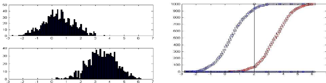
2.8 (b) Threshold calculation at maximum distances CDF
