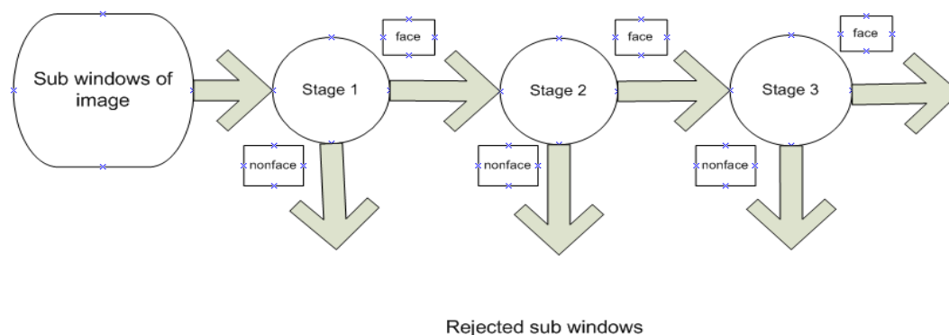
Figure 3.8: The Cascade Classifier structure.
