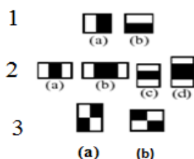
Figure 3.3: The Haar features that are used in this thesis.
